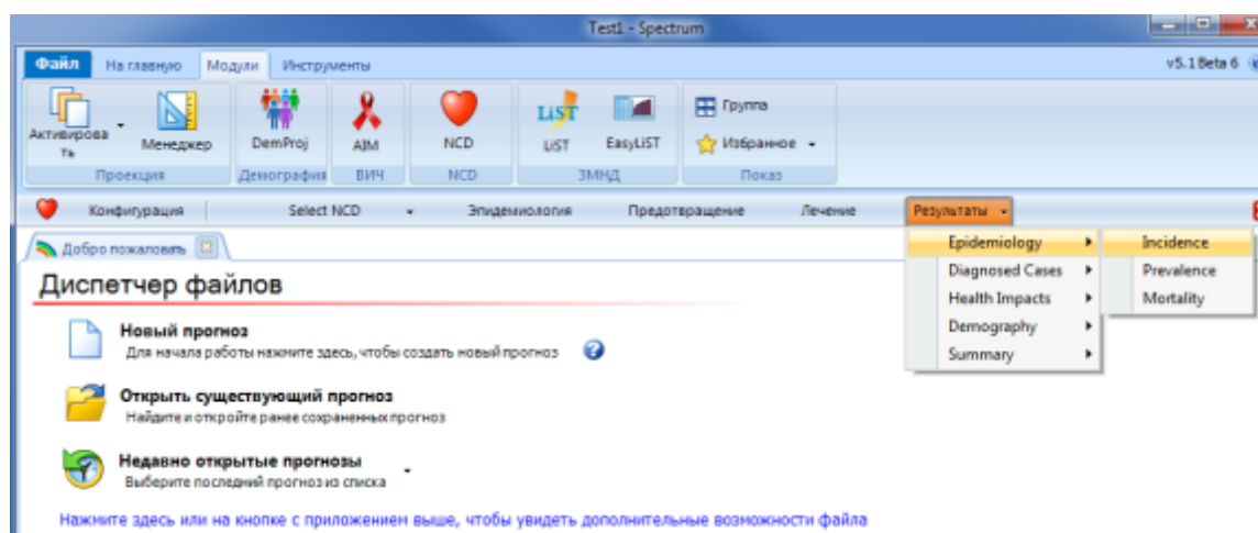
Figure 4: Generating results
